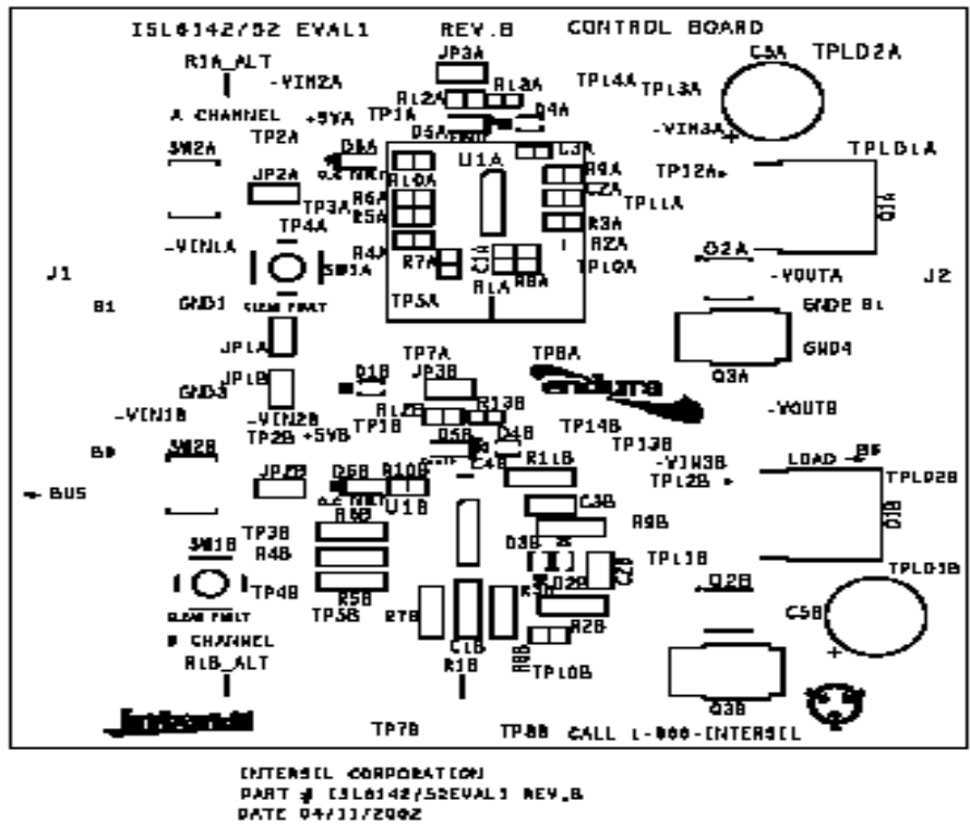
FIGURE 10. CONTROL BOARD
